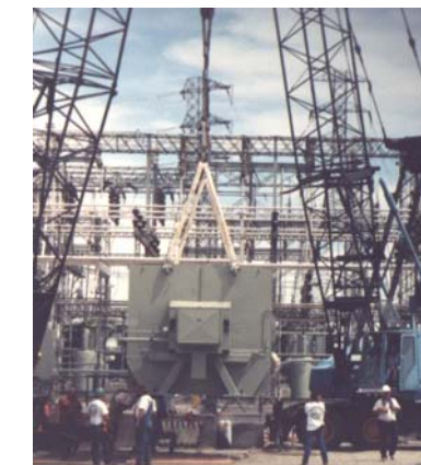
Magnetech installed new synchronous condensers for Pacific Gas & Electric. Ongoing Maintenance provided since initial installation.
