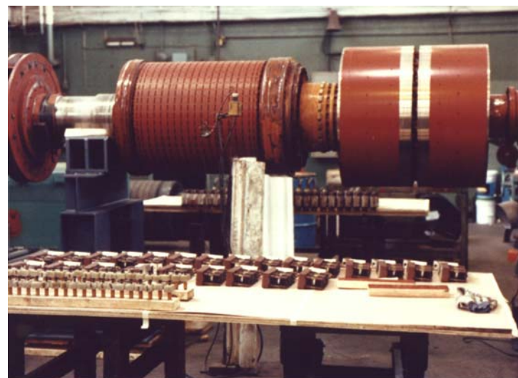
Westinghouse 4400 kW, 3600 rpm, 535 V brushless exciter with diodes and fuses rebuilt for electric utility..
